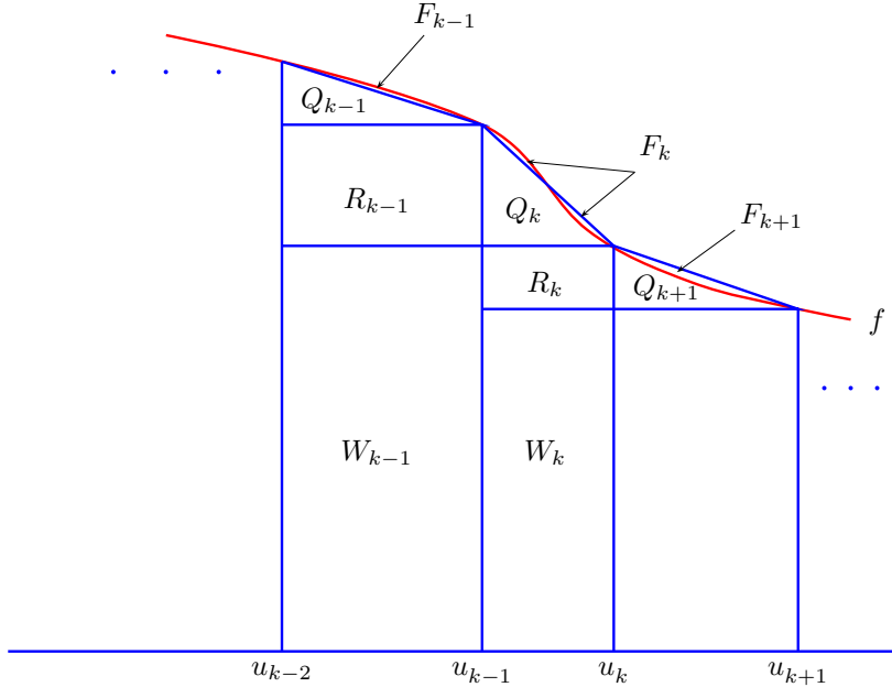
Figure 3: The dissection of \mathcal{D} .
